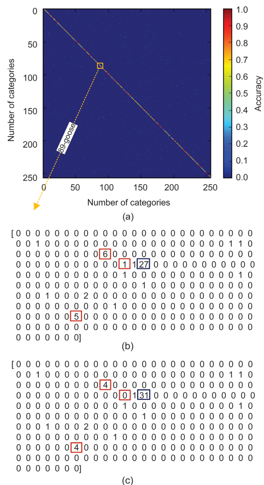
Fig. 3 The confusion matrix showing that the highly similar categories are easily misclassified: (a) the confusion matrix is generated by the result of pre-classification; (b) the classification result of category 89-goose is extracted from the confusion matrix (the number with a blue box indicates that the sample number is classified correctly and the number with a red box indicates that the sample number is misclassified); (c) the classification result of category 89-goose is extracted from the confusion matrix after using our proposed method (the sample number of misclassification among the highly similar categories is significantly reduced). References to color refer to the online version of this figure
