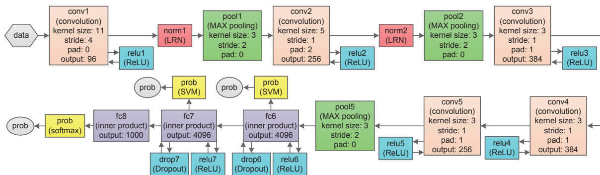
Fig. 2 Network structure of the deep CNN model. It is composed of five convolutional layers (conv1–conv5), two fully connected layers (fc6 and fc7), and a softmax output layer (Krizhevsky et al. , 2012). Layer fc6 or fc7 is commonly used to extract the deep features
